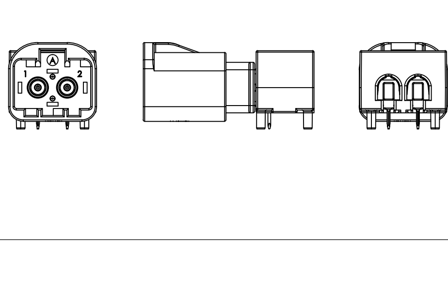
Locking Nose at 12 o'clock (e.g. 230B-P0X01)
