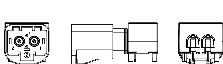
Locking Nose at 6 o'clock (e.g. 230B-P6X01)
