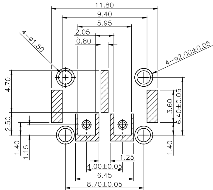
Recommended Layout (Top View) General tolerance: ±0.05mm
