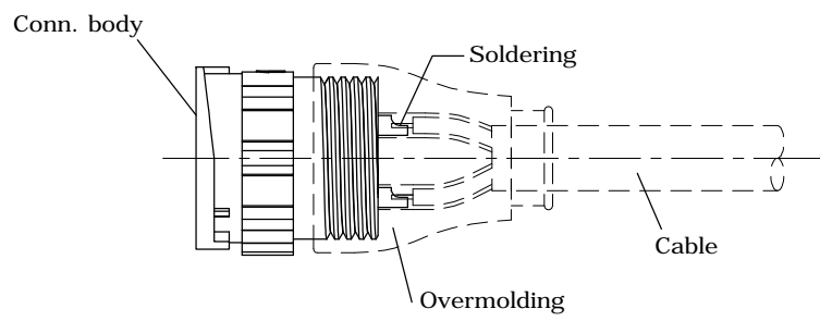
Cable overmolding, bayonet lock, female gender female pin, solder bucket
