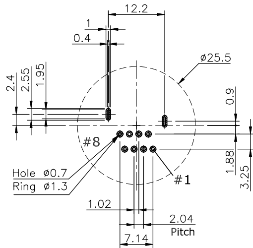
Recommended Layout ( top veiw) General Tolerance: ±0.10mm
