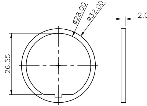
O-RING
