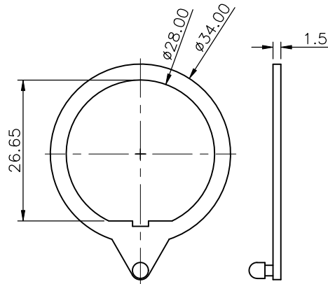
WASHER
