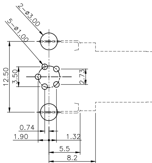
RECOMMENDED LAYOUT (TOP VIEW) GENERAL TOLERANCE: \pm 0.1\text{mm}
