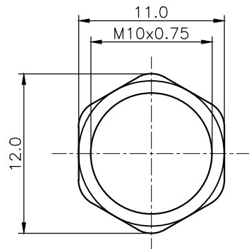
HEX-NUT
