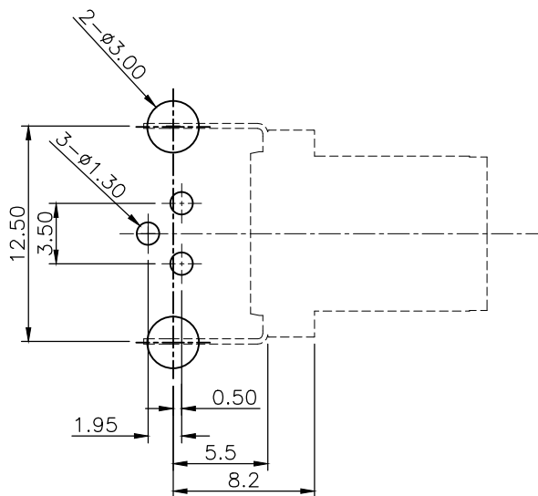
RECOMMENDED LAYOUT (TOP VIEW) GENERAL TOLERANCE: \pm 0.1\text{mm}
