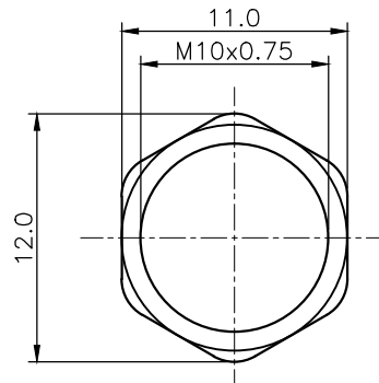
HEX-NUT
