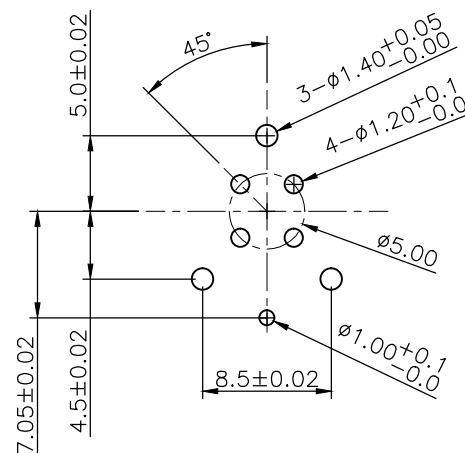
Recommended Layout (Top View) PCB Thickness: 1.6mm General Tolerance: ±0.05mm
