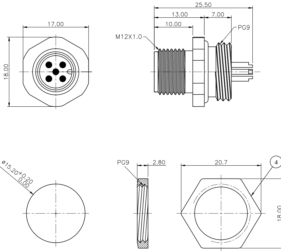
PANEL CUT-OUT
