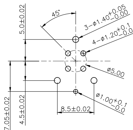
Recommended Layout (Top View) PCB Thickness: 1.6mm General Tolerance: ±0.05mm
