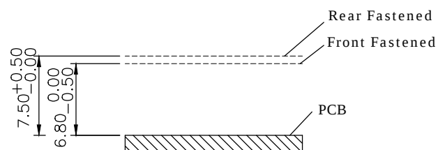
Recommended Panel Distance
