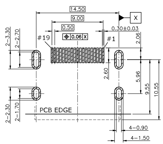
RECOMMENDED LAYOUT (TOP VIEW) GENERAL TOLERANCE: ±0.05mm
