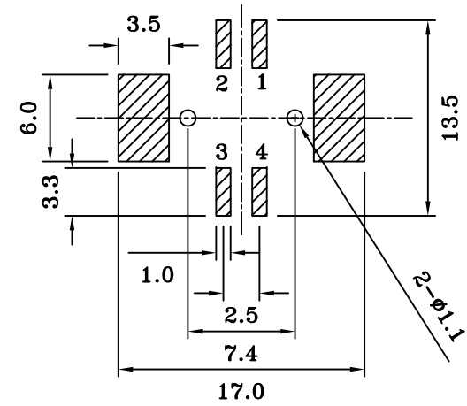
(COMPONENT SIDE) PCB LAYOUT
