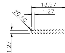
Recommended Layout General Tolerance: \pm 0.05\text{mm}
