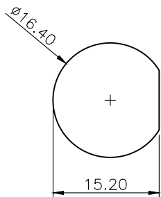
Recommended Panel Cut
