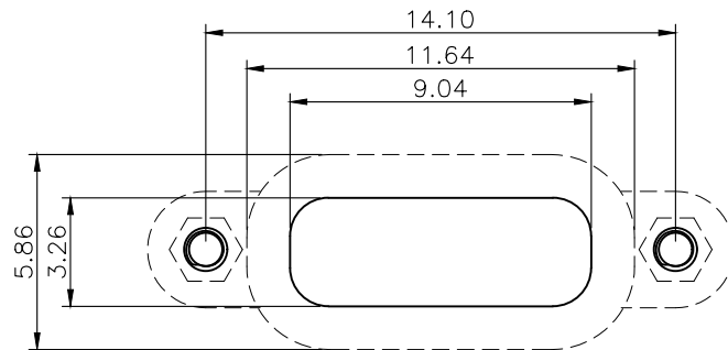
RECOMMENDED PANEL CUT
