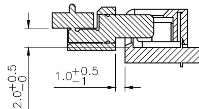
Side Insertion
