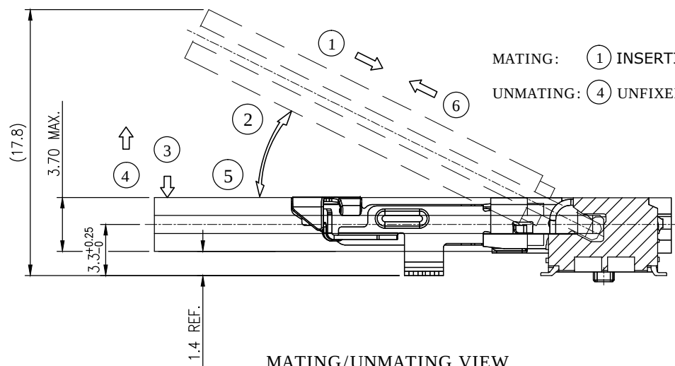
MATING/UNMATING VIEW
