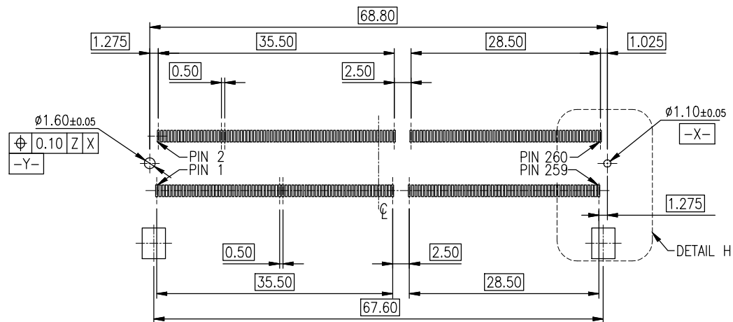
RECOMMENDED LAYOUT (TOP VIEW) GENERAL TOLERANCE: \pm 0.05
