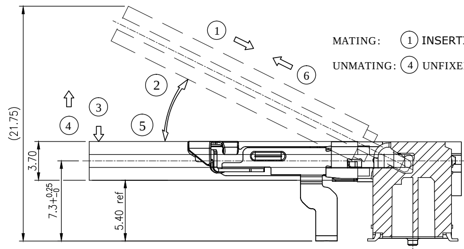
MATING/UNMATING VIEW
