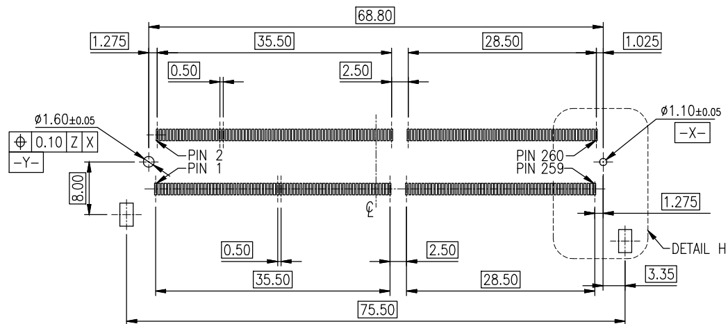
RECOMMENDED LAYOUT (TOP VIEW) GENERAL TOLERANCE: \pm 0.05
