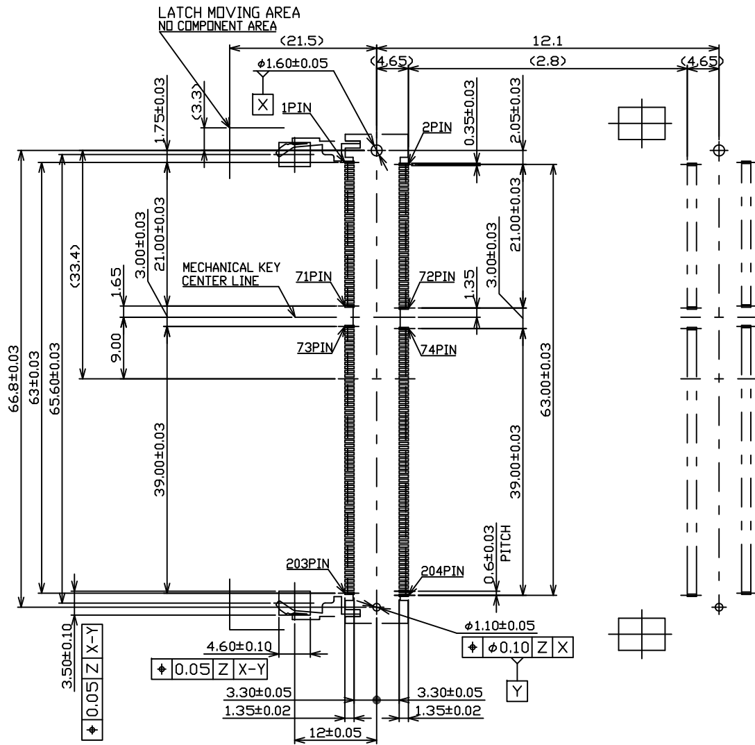
RECOMMENDED MOUNTING P.C. BOARD PATTERN LAYOUT DIM.
